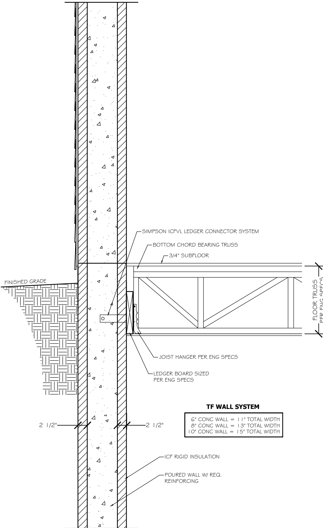
WALL SECTION (TYP.)
